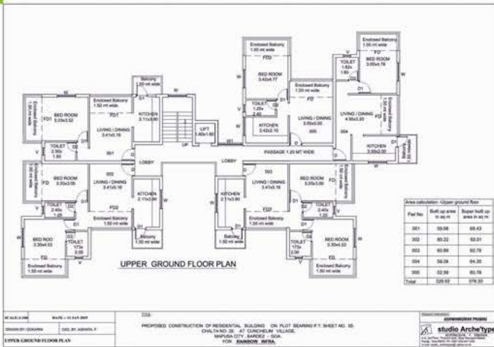
Typical Upper Ground, First Floor, & Second Floor Plan
